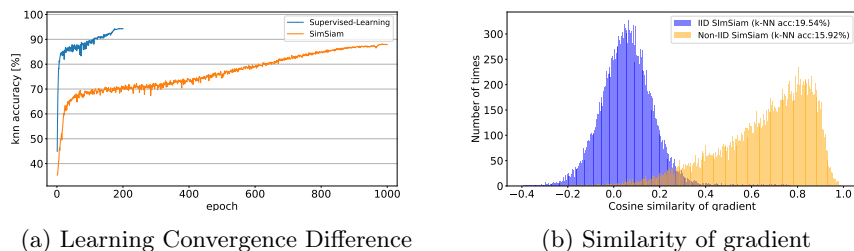
Fig. 2: Problems in Self-Supervised Online Continual Learning. (a) The k-NN accuracy during CIFAR-10 learning with SSL method SimSiam and supervised learning. The supervised learning is trained for 200 epochs, and SimSiam is trained for 1,000 epochs, with the k-NN accuracy measured for each epoch. (b) Similarity of the gradients during parameter updates in the t_{th} and (t + 1)_{th} iterations. CORE50 dataset (IID) and Seq-CORE50 (non-IID) are trained using the SSL method SimSiam.
