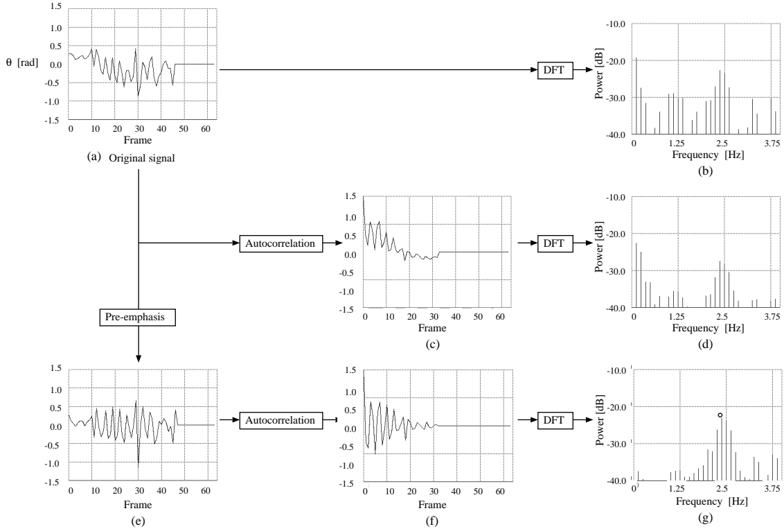
Figure 7: Process for detecting cyclic motion.
