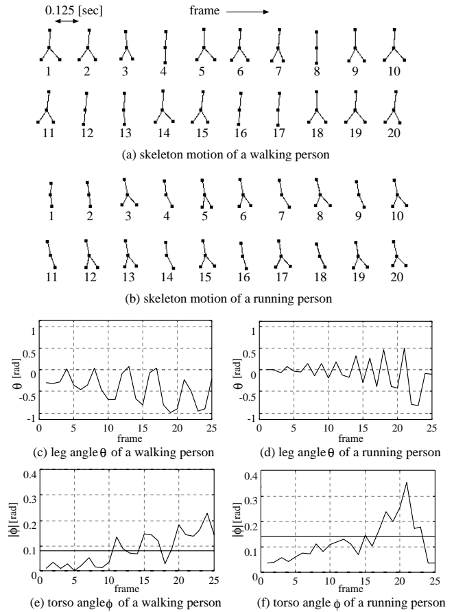
Figure 6: Skeleton motion sequences. Clearly, the periodic motion of \theta_n provides cues to the target's motion as does the mean value of \bar{\phi}_n .
