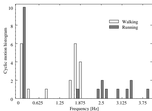
(a) Autocorrelation + DFT
